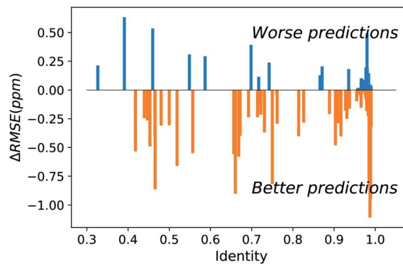
Fig. 2 Difference between UCBSHIFT-Y and SHIFTY+ for protein specific RMSEs for amide hydrogens as a function of sequence identity. The presence of more negative values indicates UCBSHIFT-Y is making better predictions than SHIFTY+ across the range of sequence identity. The better RMSE even at low sequence identity arises from finding a structural homolog.
