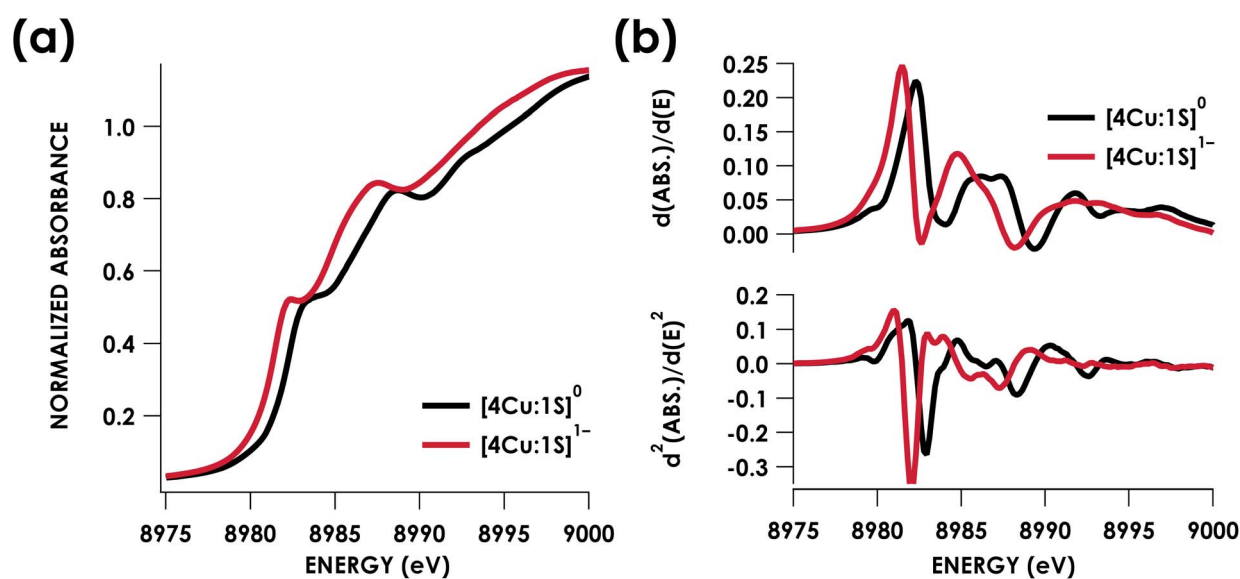
Fig. 3 (a) Cu K-edge XAS spectra obtained for the [\text{4Cu:1S}]^{0/1-} redox couple. (b) First (top) and second (bottom) derivative Cu K-edge XAS spectra. Isoenergetic pre-edge ( 1s \rightarrow 3d ) excitations are evident in the second-derivative spectra at 8979.8 eV. Rising edge inflection points occur at 8982.3 and 8985.9 eV for [\text{4Cu:1S}]^0 and 8981.5 and 8984.8 eV for [\text{4Cu:1S}]^{1-} .
