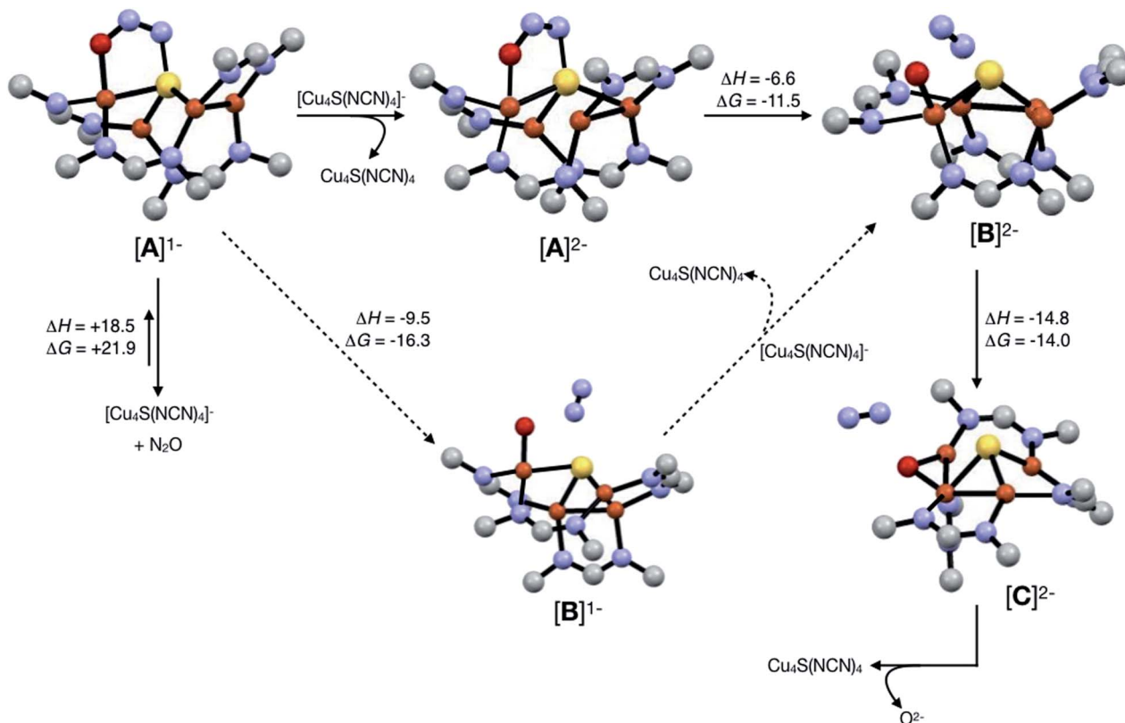
Scheme 3 Reaction pathways modeled by DFT (B3LYP/6-31G(d)). Energies at 298 K are shown in \text{kcal mol}^{-1} . The favored pathway is shown with solid arrows, and the disfavored pathway with dotted arrows.
