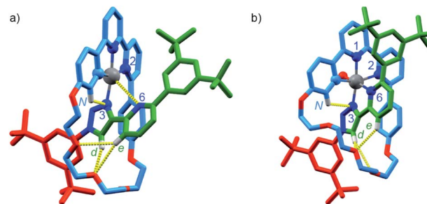
Fig. 3 Solid-state structures of (a) [Pt(k^4-4)]BF_4 and (b) [Pt(k^5-4)(OH)](SbF_6)_2 in partial sticks (rotaxane framework)/ball-and-stick (metals and ligand sphere) representation (anions and majority of hydrogen atoms omitted for clarity). Colours: H white, C as in Scheme 2, N dark blue, O red, Pt dark grey. [Pt(k^4-4)]BF_4 selected distances (Å) and angles ( ^\circ ): Pt–C 1.97, Pt–N1 1.95, Pt–N2 2.17, Pt–N3 2.03, Pt–N6 3.39, H_d –O 2.25, H_e –O 2.79, H_e –O 2.80, H_N –N 2.55, C–Pt–N2 160.7, N1–Pt–N3 172.0, C–Pt–N1 82.1, N1–Pt–N2 78.8, N2–Pt–N3 107.3, N3–Pt–C 91.6. [Pt(k^4-4)(OH)](SbF_6)_2 selected distances (Å) and angles ( ^\circ ): Pt–C 2.01, Pt–N1 1.99, Pt–N2 2.22, Pt–N3 2.01, Pt–N6 2.13, Pt–O 1.97, H_d –O 2.49, H_d –O 2.76, H_e –O 2.55, H_N –N3 2.54, C–Pt–N2 160.3, N1–Pt–N3 172.6, N6–Pt–O 171.6, C–Pt–N1 82.4, N1–Pt–N2 77.9, N2–Pt–N3 108.2, N3–Pt–C 91.4.
