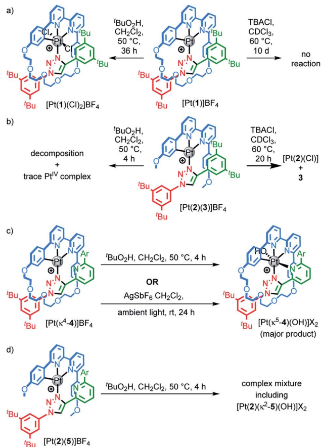
Scheme 2 Reactions of (a) [Pt(1)]BF_4 , (b) [Pt(2)(3)]BF_4 , (c) [Pt(k^4-4)]BF_4 and (d) [Pt(2)(5)]BF_4 . Ar = 3,5-di- t Bu- C_6H_3 .
