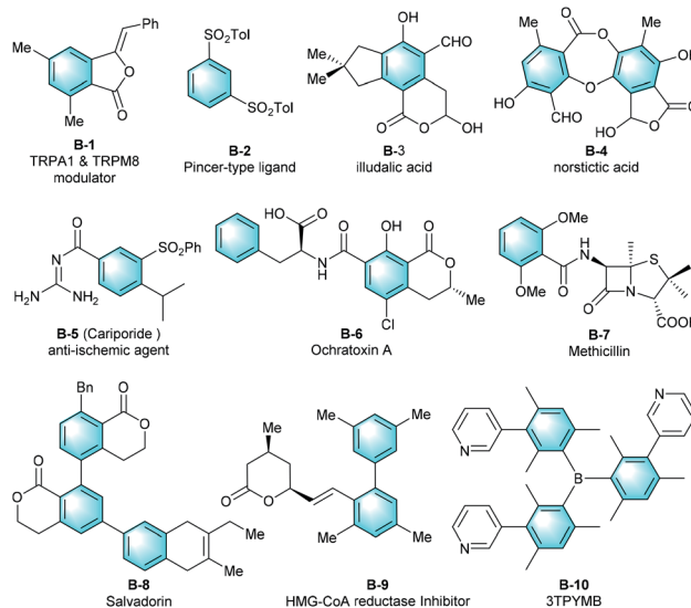
Fig. 1 Examples of multi-substituted benzenes.
