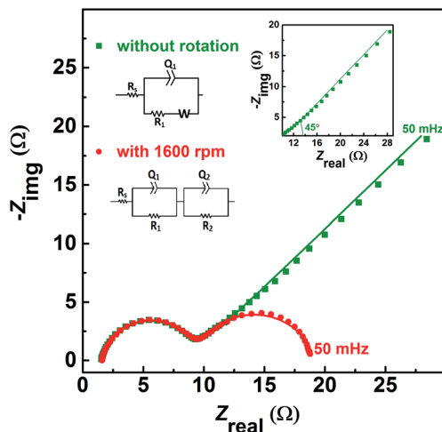
Fig. 2 EIS patterns recorded at EP on carbon-modified GCE without rotation and with 1600 rpm in equimolar (0.2 M) concentration of \text{V}^{4+} and \text{V}^{5+} in 3 \text{ M H}_2\text{SO}_4 electrolyte. The symbols and solid lines show the experimental and the fitted data, respectively. The corresponding ECs are shown in the insets. The expanded view of the 45^\circ line is shown in the inset.
