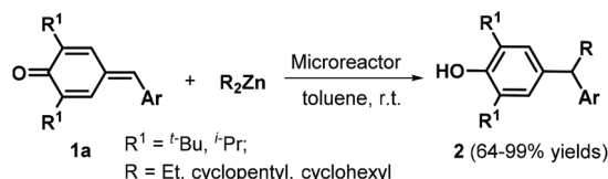
Scheme 1 1,6-Addition of dialkylzinc reagents to p -QMs.
