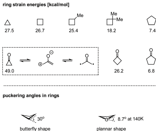
Fig. 1 Comparison of ring strain energies and structural properties of strained carbocycles.
