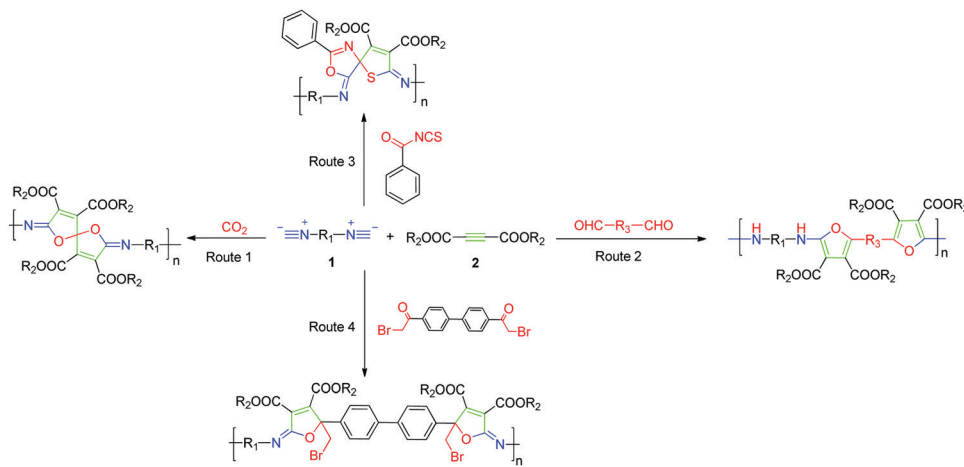
Fig. 14 MCCs based on isocyanides, DAAD, and third component.
