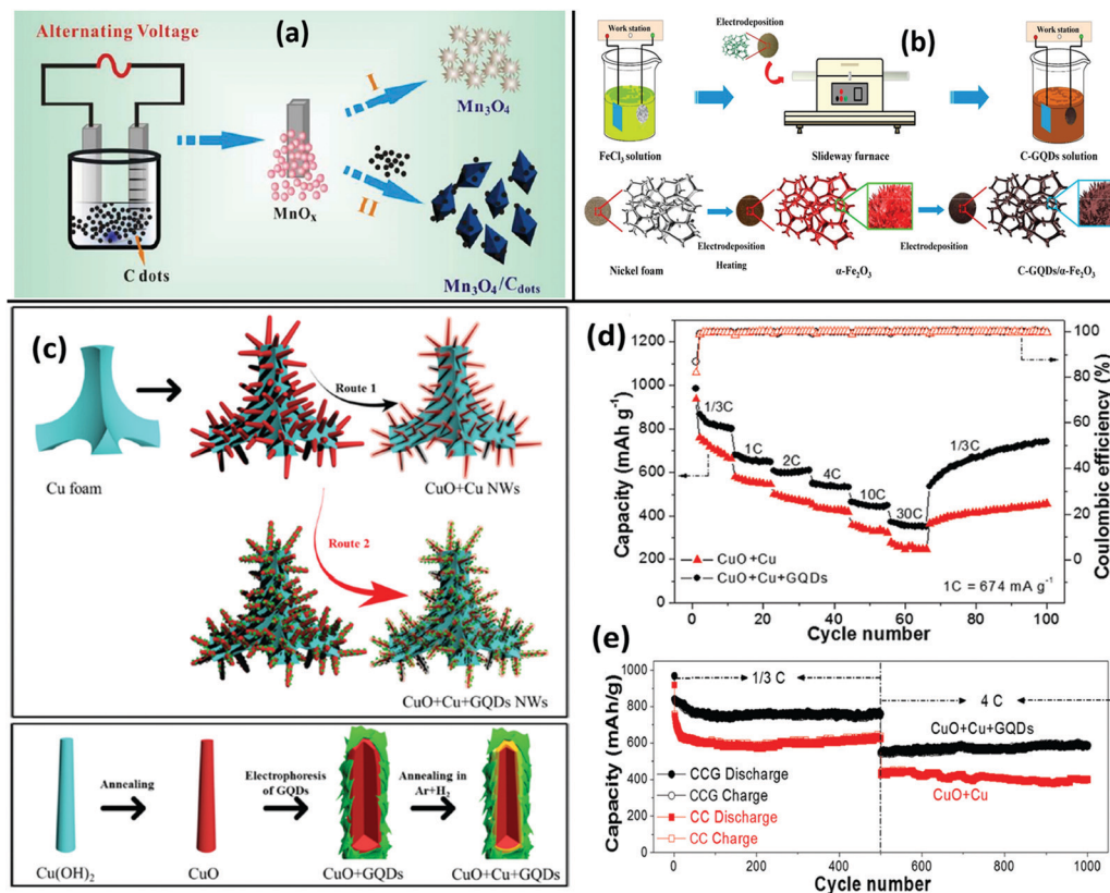
Fig. 8 (a) Schematic representation of Mn_3O_4 and Mn_3O_4/Cdots composite. Reprinted with permission from ref. 81. Copyright 2015, Royal Society of Chemistry. (b) Preparation of C-GQDs/ \alpha-Fe_2O_3 composites. Reprinted with permission from ref. 85. Copyright 2019, Elsevier. (c) Schematic of the fabrication process of CuO-based nanowire electrodes. Route 1 is for CuO + Cu (CC) core/shell nanowires. Route 2 is for CuO + Cu + GQD (CCG) triaxial nanowires; electrochemical characterization of CCG and CC anodes; (d) rate performance with coulombic efficiency; (e) cycling performance at 1/3C for the first 500 cycles and 4C for the second 500 cycles. Reprinted with permission from ref. 84. Copyright 2014, Wiley-VCH.
