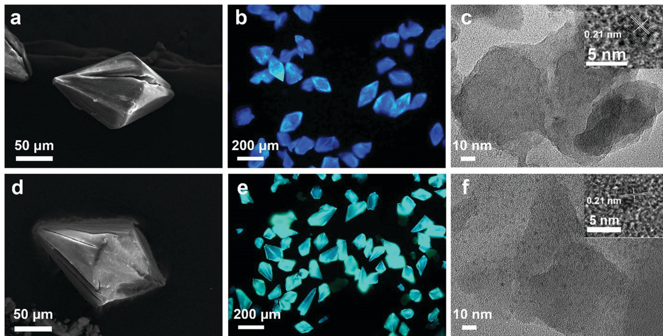
Fig. 1 (a and d) SEM images of the \text{CD}_1@MgAPO-5 and \text{CD}_1\text{CD}_2@MgAPO-5-c composites, respectively. (b and e) Fluorescence microscopy images of \text{CD}_1@MgAPO-5 and \text{CD}_1\text{CD}_2@MgAPO-5-c upon UV light excitation, respectively. (c and f) TEM images of the \text{CD}_1@MgAPO-5 and \text{CD}_1\text{CD}_2@MgAPO-5-c composites, respectively (inset, HRTEM images of CDs from the mother liquid with a lattice spacing of 0.21 nm).
