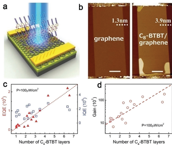
Fig. 9 (a) Schematic illustration of a typical C 8 -BTBT-graphene phototransistor. (b) The AFM images of a graphene FET before (left) and after (right) C 8 -BTBT epitaxial growth. The device is mostly covered with 1L + 1L C 8 -BTBT as reflected from the measured height increase by 2.6 nm. Scale bars: 2 μm. (c) EQE (red triangles) and IQE (blue squares) as a function of average number of C 8 -BTBT layers for all the measured devices (laser power, 100 μW cm -2 ). The red dashed line reflects the linear increase of EQE. (d) Photoconductive gain ( G_{ph} ) as a function of average number of C 8 -BTBT layers for all the measured devices (laser power, 100 μW cm -2 ). The red dashed line reflects the exponential increase of G_{ph} . Copyright 2016, Advanced Materials. 42
