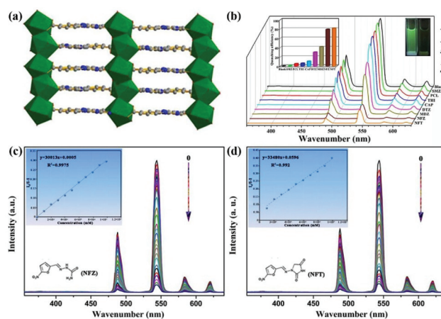
Fig. 8 (a) The 3D structure of Tb-MOF. (b) Emission spectra and optical images under UV lamp of Tb-MOF in different antibiotics. (c, d) Emission spectra of Tb-MOF and Stern–Volmer plots of (I_0/I - 1) and NFZ or NFT concentrations. Reproduced from ref. 97 with permission from the American Chemical Society.
