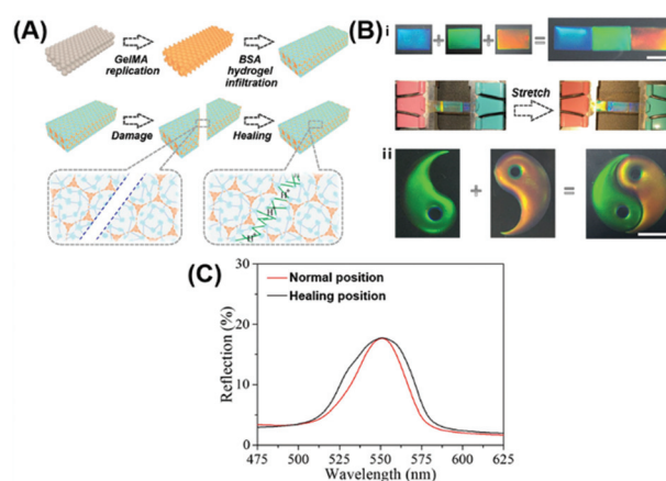
Fig. 3 Healable structural color nanocomposite via an infusion of healable polymeric materials into an ordered inverse opal structure. (A) Preparation of the structural color hydrogel material and its healing process. (B) Optical images of the healing process of structural color hydrogels. The scale bars for (i) and (ii) are 5 mm. (C) Reflection spectra of the original and healed structural color hydrogel at the damage position. Reproduced from ref. 78 with permission from the National Academy of Sciences, copyright 2017.
