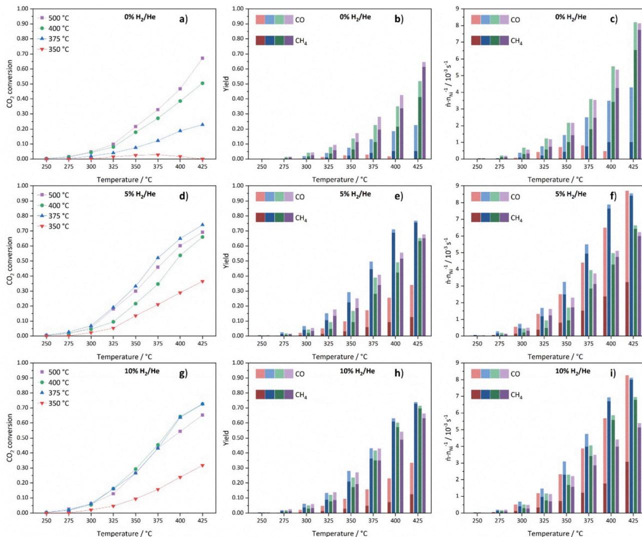
Fig. 12 CO 2 conversions (a, d and g), stacked CH 4 and CO yields (b, e and h) and stacked productivities of CH 4 and CO normalized to the molar Ni content (c, f and i) of Ni@C-5%H 2 (PNO) decomposed at temperatures of 350 °C (red), 375 °C (blue), 400 °C (green) and 500 °C (purple) in 0% (a–c), 5% (d–f) and 10% H 2 /He (g–i) atmospheres.
