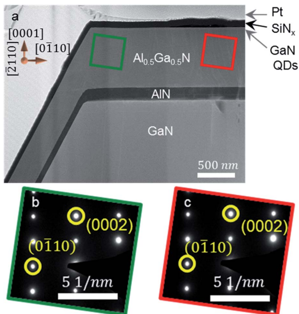
Fig. 4 (a) Cross-sectional view HAADF STEM image taken near the boundary region of the truncated pyramid structure. (b and c) SAD pattern images of the Al x Ga 1-x N layers below B- and P-QDs, respectively. Note that the SiN x and Pt layers are deposited to protect the GaN QDs layers when preparing a STEM specimen.
