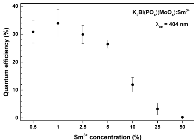
Fig. 7 Quantum efficiencies of K 2 Bi(PO 4 )(MoO 4 ):Sm 3+ phosphors as a function of Sm 3+ concentration.
