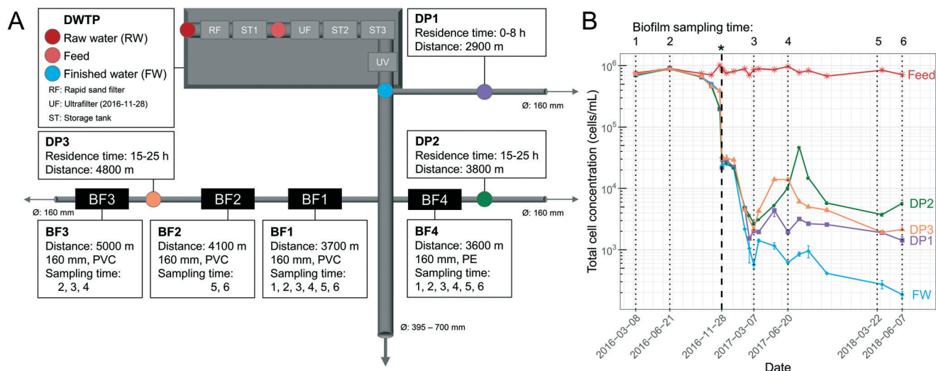
Fig. 1 Overview of sampling locations and total cell concentrations (TCC) over time. (A) Schematic illustration of the drinking water treatment plant (DWTP) process steps, and distribution points (DPs) in the DWDS, indicating locations where water was sampled, as well as biofilm (BF) points, where pipe sections were excavated for biofilm sampling. \varnothing indicates pipe diameter, arrows indicate water flow direction, and pipe material was polyethylene (PE) or polyvinyl chloride (PVC). The ultrafilter (UF) started November 28, 2016. (B) TCC in the water, determined by flow cytometry, and indicating in time when biofilm was sampled (dotted lines) and the UF start (*, bold, dashed line). Error bars show standard deviations of technical triplicates. Before the UF start, raw-water (RW) is labelled "Feed". Parts of this data are also shown in Chan et al. (2019) 11 and Schleich et al. (2019). 21
