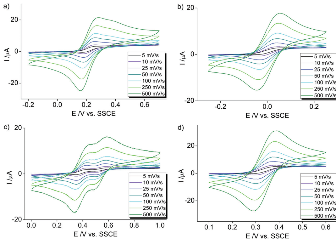
Fig. 5 Cyclic voltammetry measurements of homoleptic [\text{Co}(\text{pyPYA}_2)_2](\text{PF}_6)_2 complexes in MeCN: (a) 2a [\text{Co}(\textit{para}\text{-pyPYA}_2)_2](\text{PF}_6)_2 ; (b) 2b [\text{Co}(\textit{meta}\text{-pyPYA}_2)_2](\text{PF}_6)_2 ; (c) 2c [\text{Co}(\textit{ortho}\text{-pyPYA}_2)_2](\text{PF}_6)_2 ; (d) [\text{Co}(\textit{terpy})_2](\text{PF}_6)_2 . Conditions: 10 mL solvent, 1 mM sample and 100 mM (n\text{Bu}_4\text{N})\text{PF}_6 as supporting electrolyte at 5–500 \text{mV s}^{-1} scan rate (potentials vs. Ag/AgCl using the \text{Fc}^+/\text{Fc} couple as standard; E_{1/2} = +0.4319 ).
