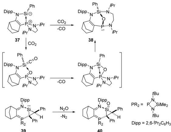
Scheme 18 Activation of \text{CO}_2 by the phosphine-stabilised silylene 37 and silacyclopent-1-ylidene 39 .
