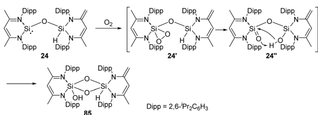
Scheme 32 Activation of the siloxysilylene 24 by O_2 .
