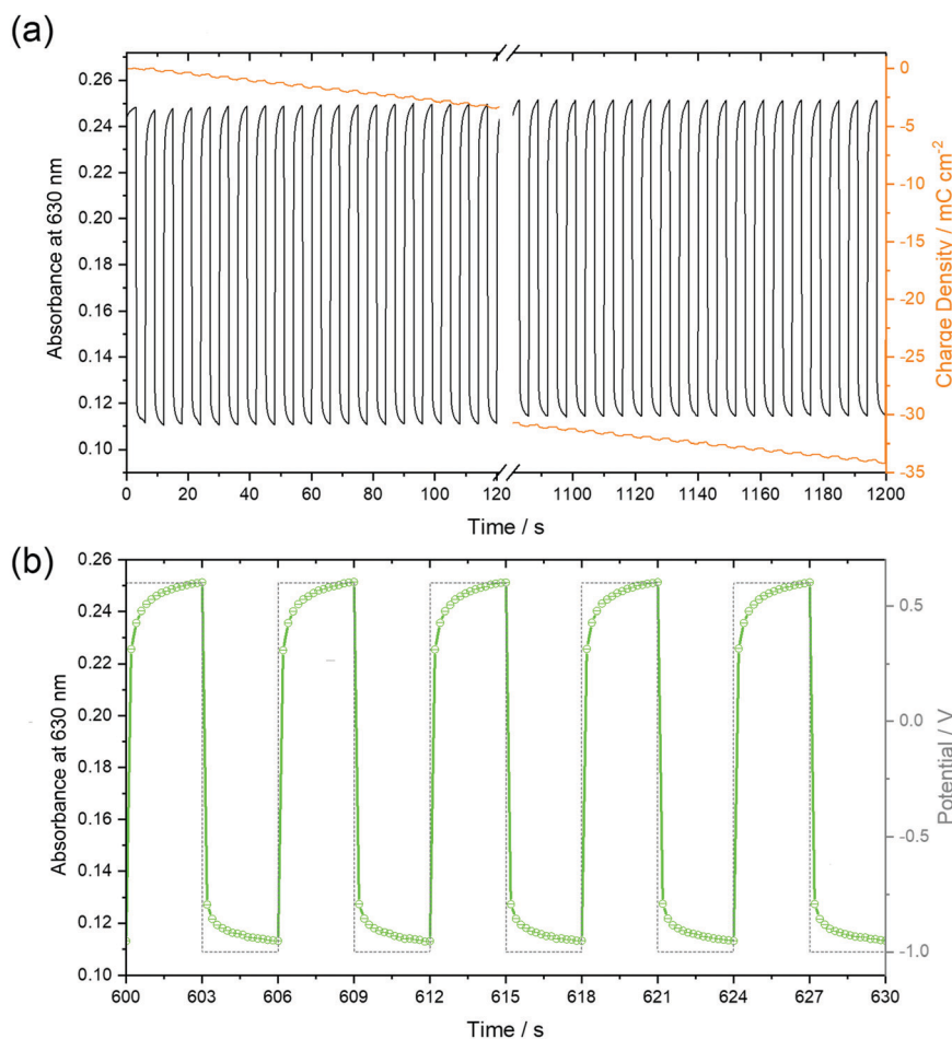
Fig. 11 Optical absorption at 630 nm of a 50 nm thin F_{40}\text{PcCu} film, recorded during chronoamperometry over 20 minutes (a) and at high resolution for an intermediate time interval (b) between the potentials depicted as dashed profiles in (b). The variation of the charge density within 200 cycles is shown as orange lines in (a).
