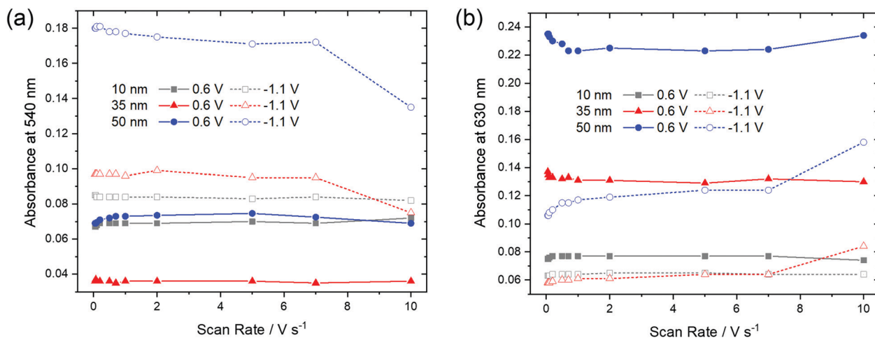
Fig. 10 Optical absorbance at (a) 540 nm and (b) 630 nm as a function of scan rate of F_{40}\text{PcCu} films of different thickness in the re-oxidized (0.6 V) or reduced (-1.1 V) states.
