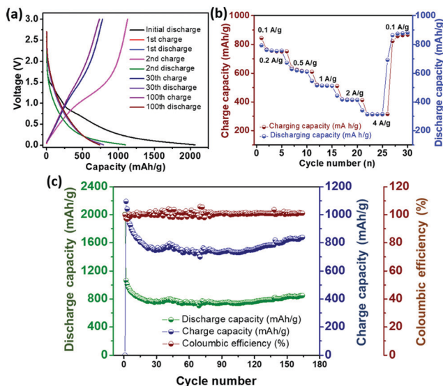
Fig. 3 (a) Discharge–charge voltage profile, (b) rate capability and (c) cycling performance of the electrode containing 3 in the half-cell w. r. t. \text{Li}/\text{Li}^+ .
