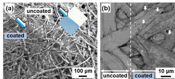
Fig. 14 Scanning electron microscopy (SEM) images of the PDA-coated papers. (a) Secondary-electron image of the PDA- Zn^{2+} -coated (lower-left part indicated by blue arrow) and uncoated (upper-right part indicated by white arrow) parts. The inset shows the photograph of the filter paper. Reprinted with permission from ref. 78. Copyright 2020 American Chemical Society. (b) Back-scattered electron image of the uncoated (left) and PDA- C_6-NH_2 coated (right) parts. Reprinted with permission from Wiley-VCH. 85
