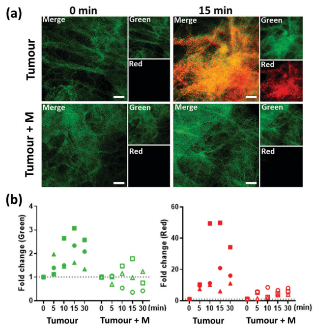
Fig. 2 Specific activation of 3 by cancerous human lung tumour tissue. Compound 3 (5 μM) was added to ex vivo human lung cancer tissue ( \pm marimastat, M). The tissue was interrogated using an optical fibre-based imaging device with 300 frames collected per time-point (0–30 min) post addition of 3 . (a) Individual frame from the 10 s video (per time-point/condition) is shown. Merge is an overlay of the two fluorescent channels, which are shown individually within the inserts. (b) Fold-change in average fluorescence (FAM: green and Cy5.5: red) after incubation with the compound was compared to base-line fluorescence from the two channels. At each time point, the mean intensity of the 300 video frames is shown. Data is from three independent patient tumour samples with each symbol representing an individual patient ( \pm marimastat, M). Scale bar is 50 μm.
