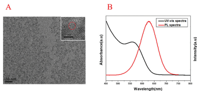
Fig. 2 (A) TEM image of CdTe QDs, (B) UV-vis spectra and PL spectra of CdTe QDs.
