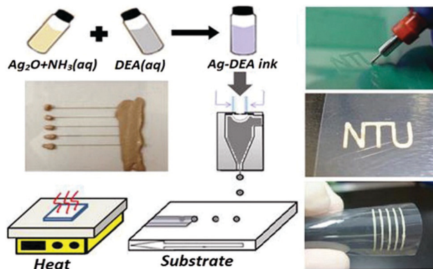
Fig. 11 The formulation, deposition and metallization processes of the ink and the images of the written silver conductive films. Reproduced with permission from ref. 68. Copyright 2012, American Chemical Society.
