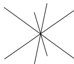
Body-Centered Cubic
