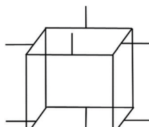
Isocube
