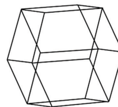
Rhombic Dodecahedron
