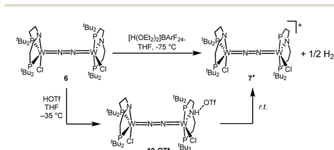
Scheme 6 Oxidation of 6 with 1 equiv. of acid at different temperatures.
