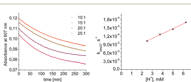
Fig. 4 Left: plot of the absorbance at 607 nm vs. time for different concentrations of [HNET_3^+] . Results from fitting to the rate law are indicated by red lines. Right: plot of k_{\text{obs}(2)} vs. [H^+] .
