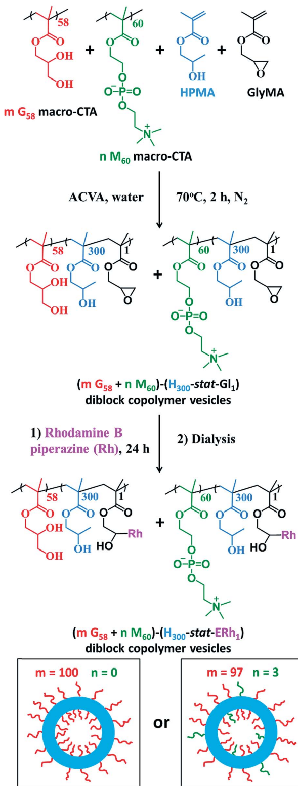
Fig. 1 Synthesis of fluorescently-labelled PGMA_{58}\text{-P(HPMA}_{300}\text{-stat-GlyMARh}_1) diblock copolymer vesicles (denoted G_{58}\text{-(H}_{300}\text{-stat-ERh}_1) , where m = 100 and n = 0 ) and (97 PGMA_{58} + 3 PMPC_{60})\text{-P(HPMA}_{300}\text{-stat-GlyMARh}_1) diblock copolymer vesicles (denoted (97 G_{58} + 3 M_{60})\text{-(H}_{300}\text{-stat-ERh}_1)\text{-D}_{52} where m = 97 and n = 3 ) via RAFT aqueous dispersion polymerization. Corresponding schematic cartoons are also shown for each type of precursor vesicle, where PGMA = red, PMPC = green, P(HPMA-stat-ERh 1 ) = blue. RAFT end-groups are omitted from chemical structures to aid clarity.
