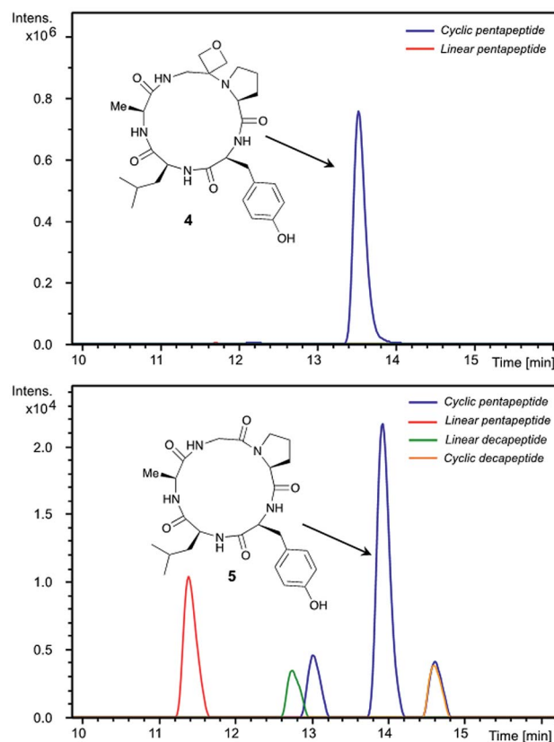
Fig. 1 Extracted ion chromatograms of peptide macrocyclisations [DEPBT (2 equiv.), ^i\text{Pr}_2\text{EtN} (2 equiv.), DMF (0.001 M), 48 h, RT] for 1 → 4 (top) and 3 → 5 (bottom).
