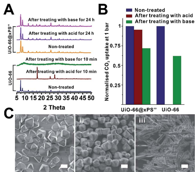
Fig. 6 PXRD patterns (A) and normalized CO 2 uptake at 195 K (B) of non-treated UiO-66 and UiO-66@xPS'' and after treating them with 1 M H 2 SO 4 and 1 M NaOH at 50 °C for different times. (C) SEM images of UiO-66 (i), UiO-66@xPS'' after treating with 1 M H 2 SO 4 for 24 h (ii), and UiO-66 after treating with 1 M H 2 SO 4 for 10 min (iii); scale bars are 1 μm for (i) and (ii), and 2 μm for (iii).
