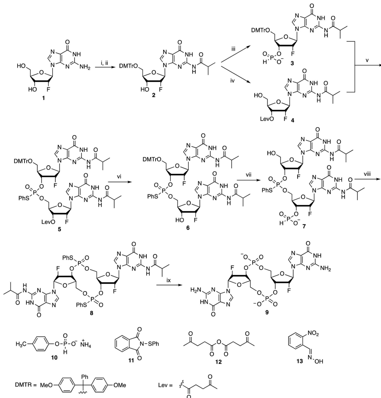
Scheme 1 Reagents and conditions: (i) (a) (CH 3 ) 3 SiCl, (CH 3 ) 2 CHCOCl, C 5 H 5 N; (b) aq. NH 3 ; (ii) DMTrCl, C 5 H 5 N; (iii) (a) 10 , (CH 3 ) 3 CCOCl, C 5 H 5 N; (b) H 2 O; (iv) (a) 12 , C 5 H 5 N; (b) Cl 2 CHCOOH, pyrrole, CH 2 Cl 2 ; (v) (a) (CH 3 ) 3 CCOCl, C 5 H 5 N; (b) 11 , C 5 H 5 N; (vi) NH 2 NH 2 ·H 2 O, CH 3 COOH, C 5 H 5 N, H 2 O; (vii) (a) 10 , (CH 3 ) 3 CCOCl, C 5 H 5 N; (b) H 2 O; (c) Cl 2 CHCOOH, pyrrole, CH 2 Cl 2 ; (viii) (a) (PhO) 2 P(O)Cl, C 5 H 5 N; (b) 11 , C 5 H 5 N; (ix) (a) 13 , TMG; (b) aq. NH 3 , 55 °C.
