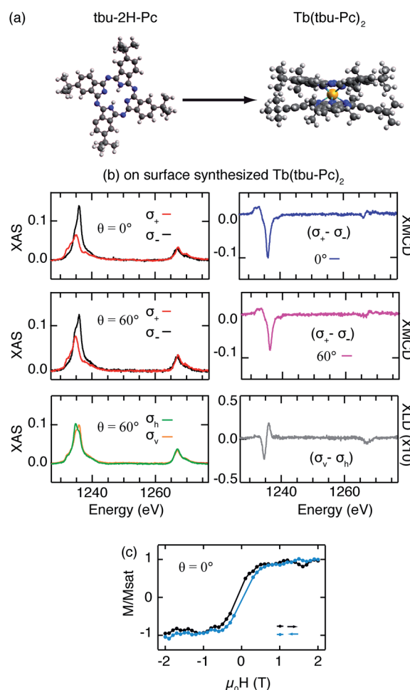
Fig. 5 (a) Schematic of tbu-2H-Pc and \text{Tb}(\text{tbu-Pc})_2 . (b) XAS, XMCD, and XLD probed at the Tb M_{4,5} edges and (c) magnetization curve probed at the Tb M_{4,5} edge (3.7 ML tbu-2H-Pc / \text{Ag}(111) + 0.8 ML Tb; \mu_0 H = 50 mT and 6.8 T for measurements with linear and circular polarizations, respectively, \mu_0 \dot{H} = 2 T \text{min}^{-1} for magnetization curves measurements, T = 3 K).
