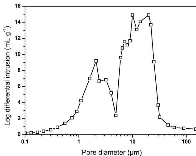
Fig. 3 Pore size distribution of sample 7.
