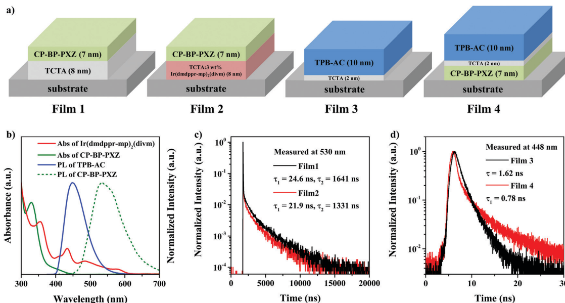
Fig. 4 (a) Structures of films 1–4. (b) Absorption spectra of the \text{Ir}(\text{dmprr-mp})_2(\text{divm}) and CP-BP-PXZ films, and PL spectra of the CP-BP-PXZ and TPB-AC films. (c) Transient PL spectra of films 1 and 2 measured at 530 nm. (d) Transient PL spectra of films 3 and 4 measured at 448 nm.
