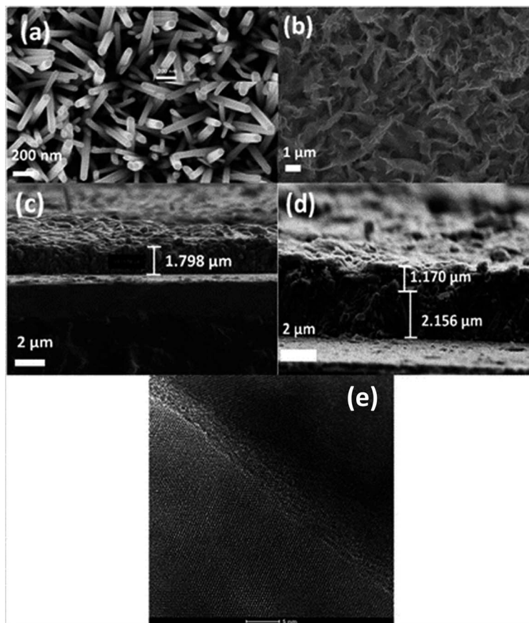
Fig. 6 (a) SEM of ZnO nanorods (0.025 M), (b) Cul (30 cycles), (c) cross section of ZnO grown on FTO, (d) cross section of ZnO/Cul on FTO, (e) heterojunction of ZnO and Cu in the composite.
