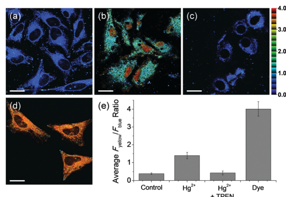
Fig. 4 Pseudo colored ratiometric TPM images of HeLa cells incubated with (a) probe NAP-PS (5 \mu M) and (d) dye ( NAP-OH , 5 \mu M) for 30 min; HeLa cells were pretreated with (b) \text{Hg}(\text{ClO}_4)_2 (25 \mu M) for 30 min and (c) \text{Hg}(\text{ClO}_4)_2 and then with TPEN (1 mM) for an additional 30 min before labeling with probe NAP-PS ; (e) average F_{\text{yellow}}/F_{\text{blue}} ratios in the TPM images. Images were acquired using 740 nm excitation and emission windows of 400–450 nm (blue) and 500–600 nm (yellow); scale bars = 20 \mu m.
