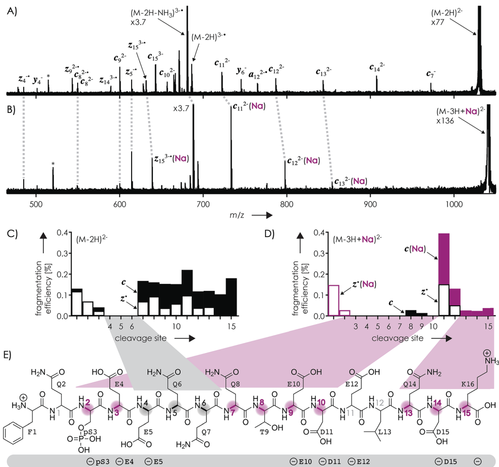
Fig. 1 Spectra from niECD of (A) (M-2H)^{2-} and (B) (M-3H+Na)^{2-} ions using a skimmer potential of 10 V (asterisks indicate harmonic signals) 70 and (C, D) corresponding site-specific fragmentation efficiency (N–C \alpha backbone bond cleavage, >98% c , z' and <2% c' , z fragments); (E) primary structure of the phosphopeptide with proposed protonation sites (N terminus and K16) and possible locations of the four negative charges (pS3, E4, E5, E10, D11, E12, D15, and the C terminus) indicated below; highlighted in gray are sites from which no fragments were observed in niECD of (M-2H)^{2-} ions, and in purple sites at which fragment ion formation was substantially reduced or prevented in niECD of (M-3H+Na)^{2-} ions.
