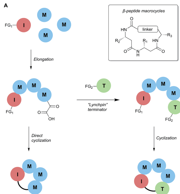
Scheme 2 Strategies to adapt synthetic fermentation methodology for the preparation of \beta -peptide macrocycles. (A) General cyclization strategies; (B) proposed 1,3,4-thiadiazole-forming reaction for macrocyclization.
