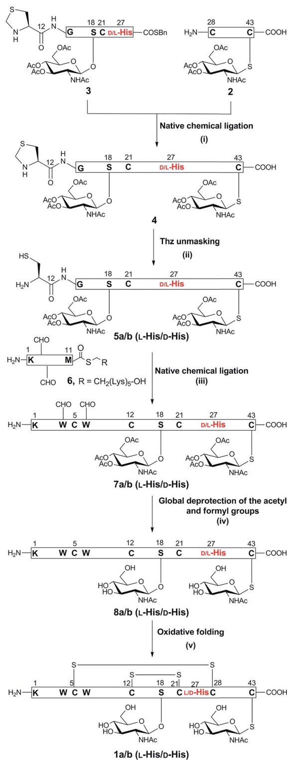
Scheme 1 Synthesis of GccF (1) and [ 27 D]-GccF, with the problematic His highlighted in red. Reagents and conditions: (i) 6 M Gn·HCl, 0.2 M Na 2 HPO 4 , 100 mM MPAA, 20 mM TCEP, pH 6.8, r.t., 2 h; (ii) 6 M Gn·HCl, 0.2 M Na 2 HPO 4 , methoxylamine·HCl, pH 4, r.t., 16 h; (iii) 6 M Gn·HCl, 0.2 M Na 2 HPO 4 , 100 mM MPAA, 20 mM TCEP, pH 6.8, r.t., 4 h; (iv) 6 M Gn·HCl, 1 M HEPES, hydrazine, 2-mercaptoethanol, 0 °C, 30 min; (v) 1.5 M Gn·HCl, 50 mM Na 2 HPO 4 , 2 mM cysteine, 0.25 mM cysteine, 0.025 mM EDTA, 0.25 mM peptide, pH 8.2, 4 °C, 16 h.
