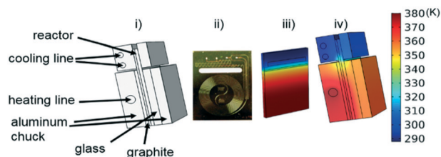
Fig. 6 (i) Labeled reactor setup (ii) microreactor (iii) simulated temperature profile of microreactor (iv) simulated temperature profile of reactor with aluminium enclosure.
