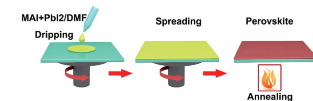
Fig. 6 One-step deposited perovskite films.
