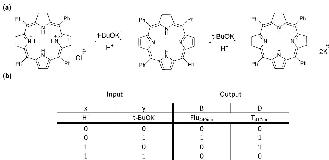
Fig. 3 (a) Three ionization states of 5,10,15,20-tetraphenylporphyrin. (b) Truth table for the molecular half-subtractor logic gate. Reproduced from ref. 5 with permission from American Chemical Society, copyright 2003.
