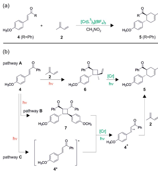
Fig. 6 (a) Diels–Alder reaction between chalcone derivative 4 and isoprene 2. 17 (b) Possible mechanistic pathways. Reproduced from ref. 17 – Published by The Royal Society of Chemistry.
