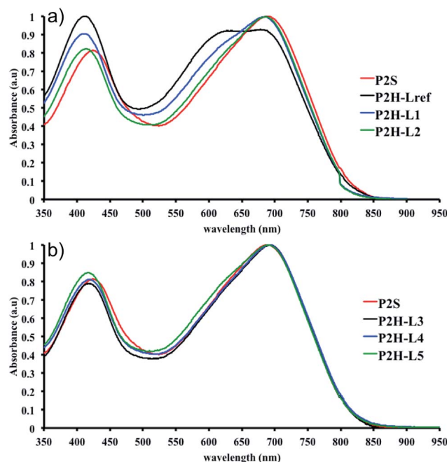
Fig. 4 UV-Vis spectra of P2S and P2H series (solution in \text{CHCl}_3 ).
