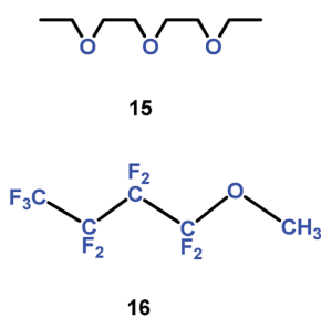
Scheme 9 The structures of organic solvent alkyl ethers. 32
