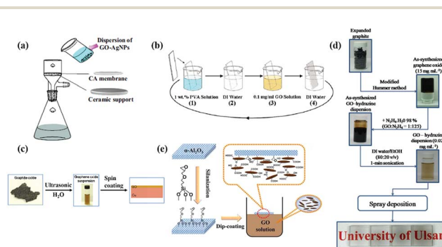
Fig. 7 (a) Vacuum filtration method; 64 (b) layer-by-layer self-assembly method (LBL); 88 (c) spin coating method; 53 (d) spraying method; 71 (e) dip coating method. 74
