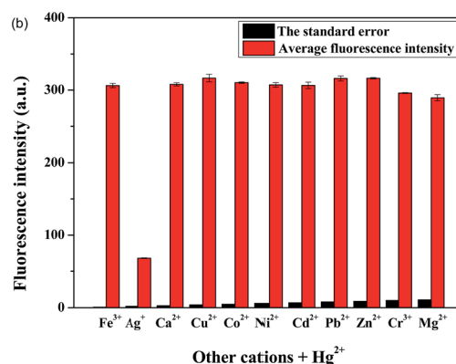
Fig. 2 (a) Fluorescence spectra of Z-3 and Z-3 + \text{Hg}^{2+} in the presence of 10 equiv. various metal ions in DMSO/ \text{H}_2\text{O} (v/v, 3 : 2; buffered with HEPES, pH = 7.20) solutions; (b) error bar of Z-3 + \text{Hg}^{2+} in the presence of various cations.
