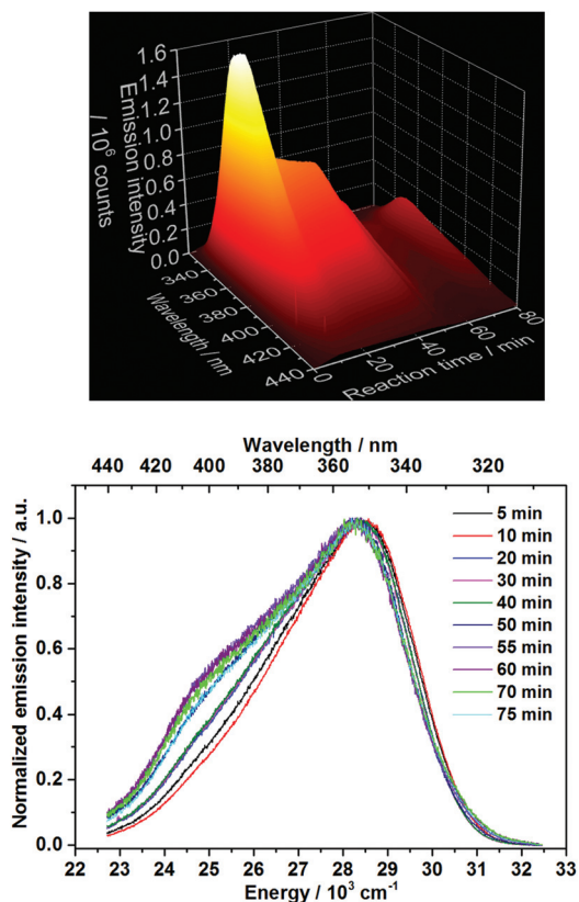
Fig. 1 Top: In situ emission spectrum recorded during calcium phosphate phase transitions applying 3% Ce 3+ as a coordination sensor (λ ex = 280 nm). Bottom: Normalized emission spectra for selected reaction times (experiment 2, Table 1).
