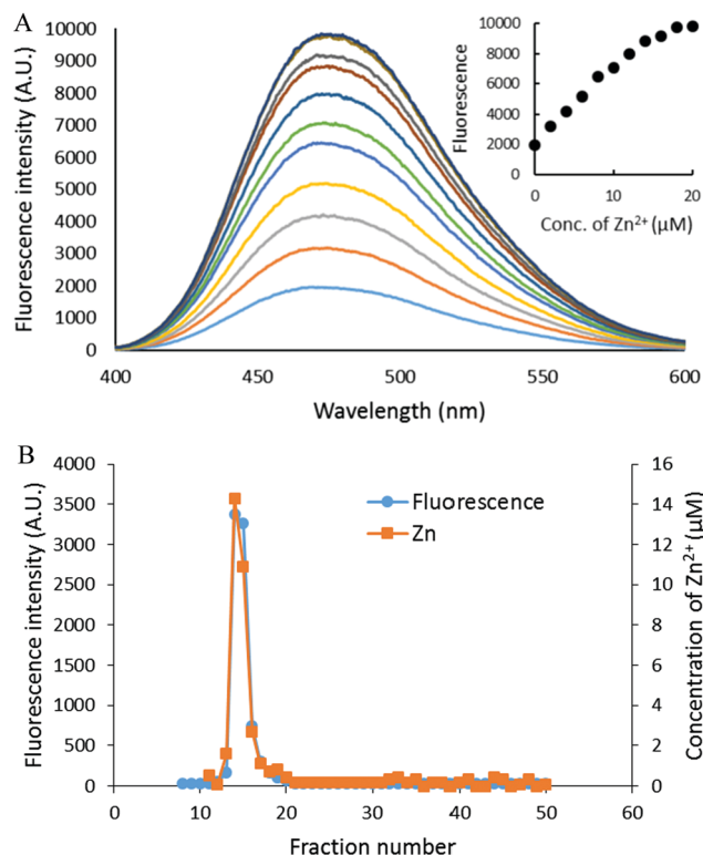
Fig. 8 \text{Zn}^{2+} titration of isolated proteome pre-treated with TSQ. (A) Isolated proteome ( 8 \mu\text{M Zn}^{2+} ) was reacted with 20 \mu\text{M TSQ} for 30 min (the bottom most spectrum). Following on, the reaction mixture was titrated with increasing concentrations of \text{ZnCl}_2 . The inset summarizes the fluorescence changes as a function of \text{Zn}^{2+} . (B) The final reaction mixture from (A) was fractionated using Sephadex G-75 gel filtration, and the eluted fractions were analyzed for both fluorescence and zinc content.
