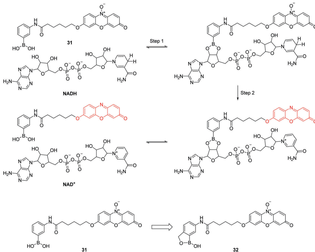
Fig. 15 Structures of 31 , 32 and proposed mechanism for detection of NADH by 31 .
